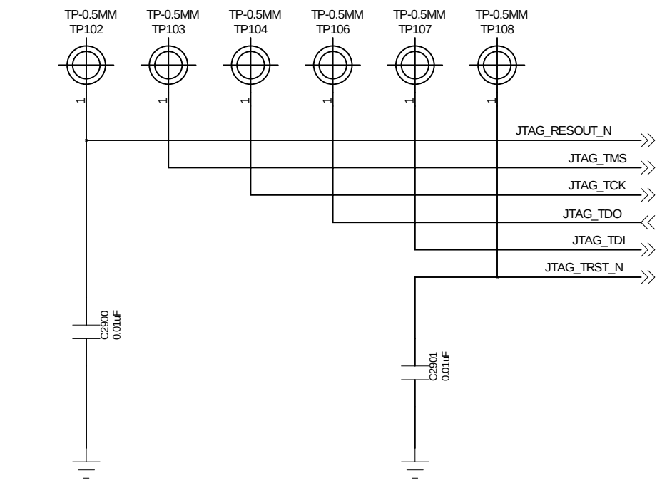
JTAG CONNECTOR
